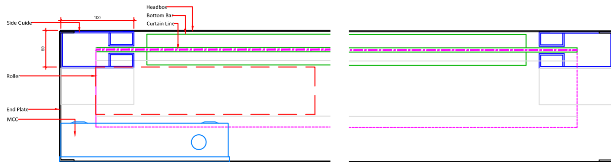
03/001 Plan Section Of Through Headbox SCALE 1:5 @ A3
