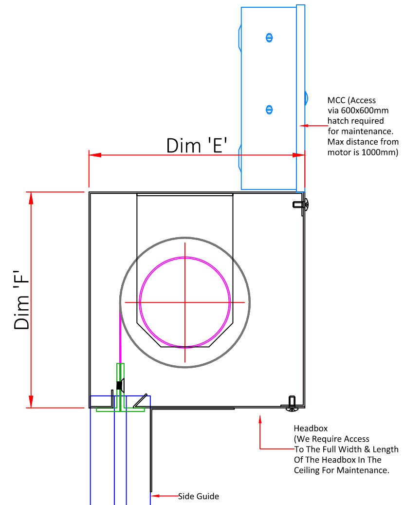
02/001 Section Through Headbox SCALE 1:3 @ A3
