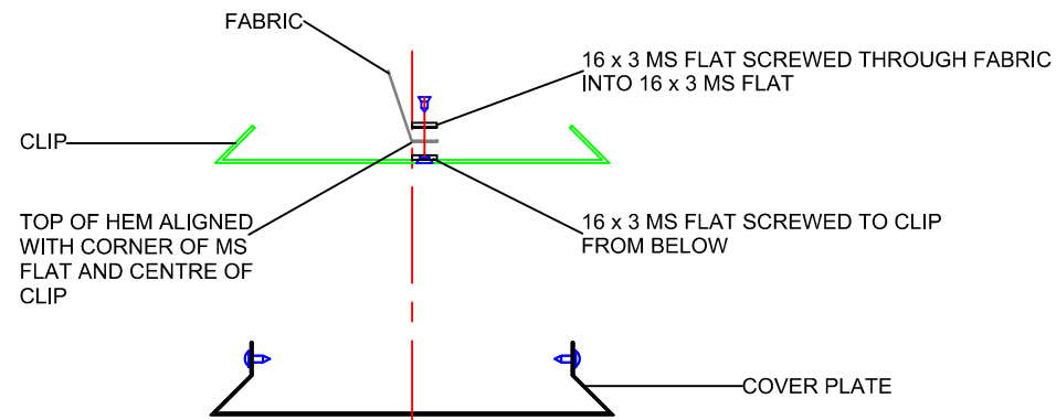
COVER PLATE ASSEMBLY
