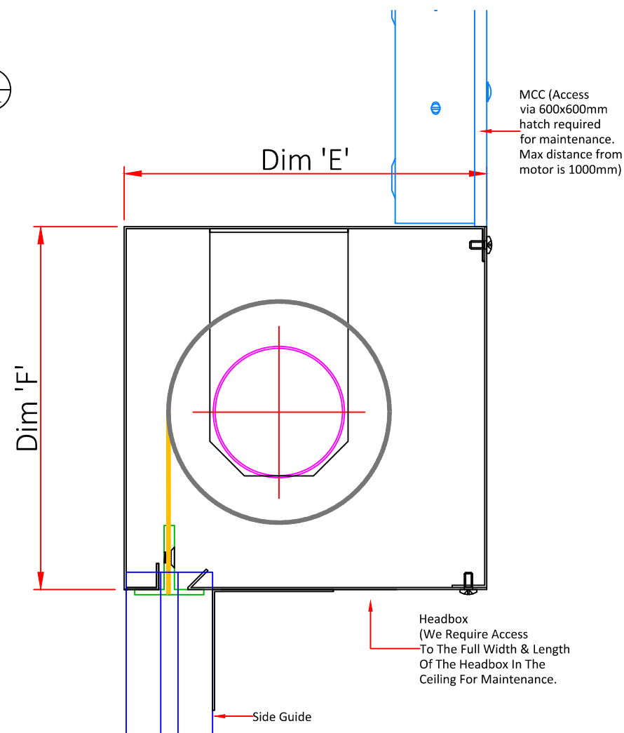
02 Section Through Headbox 001 SCALE 1 : 3 @ A3
