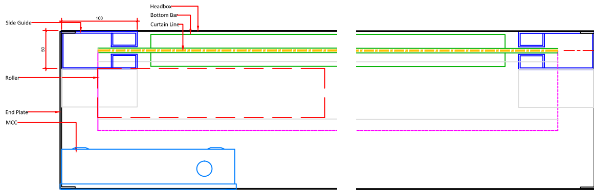
03 Plan Section Of Through Headbox 001 SCALE 1 : 5 @ A3
